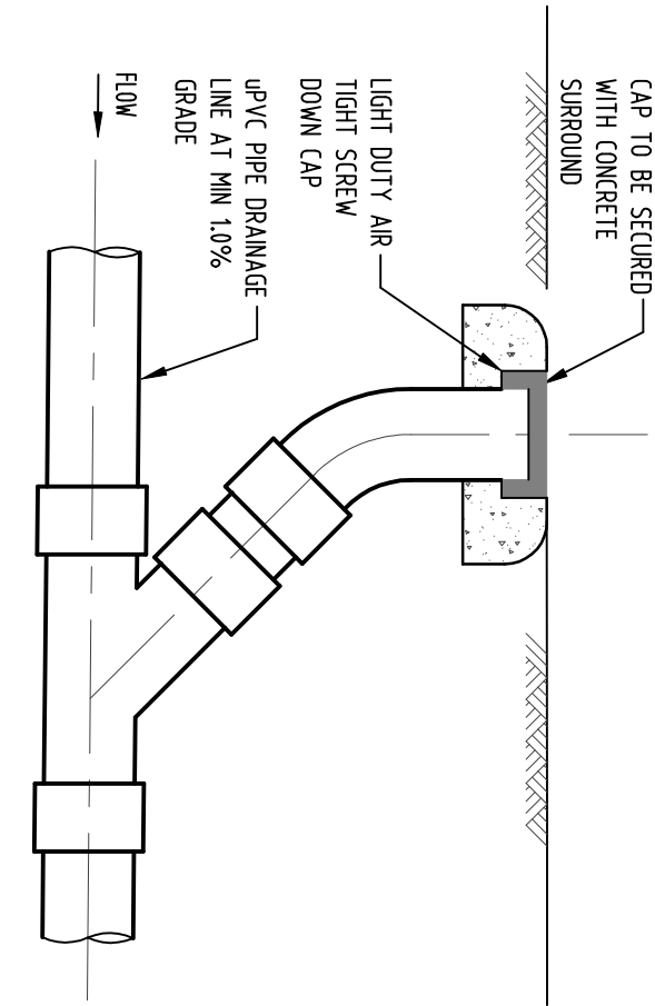
4 DETAIL CLEANING EYE SCALE 1:10
