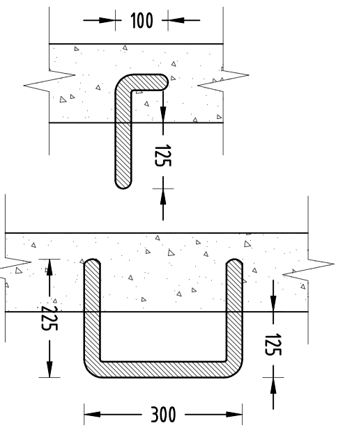
1 DETAIL STEP IRONS SCALE 1:10
